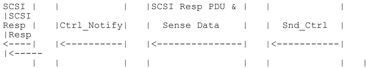
Figure 9 A SCSI Write data transfer
