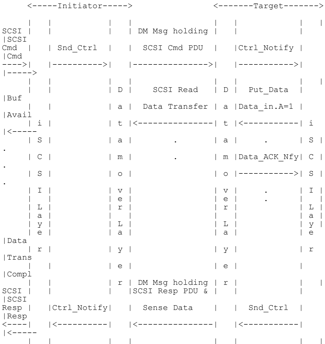
Figure 11 A SCSI Read data acknowledgement
