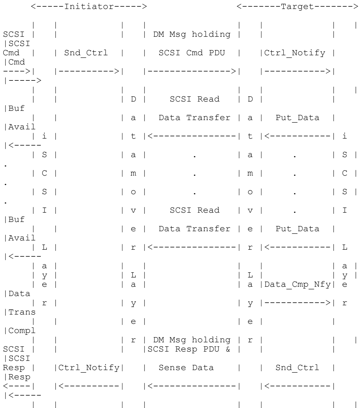
Figure 10 A SCSI Read data transfer
