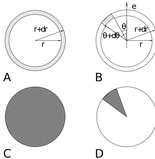
Fig. 5.52: Definition of slices in gmx rdf (page 243): A. g_{AB}(r) . B. g_{AB}(r, \theta) . The slices are colored gray. C. Normalization \langle \rho_B \rangle_{local} . D. Normalization \langle \rho_B \rangle_{local, \theta} . Normalization volumes are colored gray.
