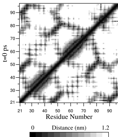
Fig. 5.57: A minimum distance matrix for a peptide 168 (page 583).
