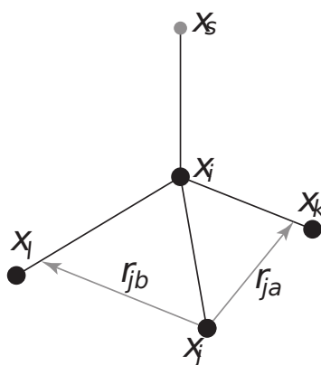
Fig. 5.36: The new 4fdn virtual site construction, which is stable even when all constructing atoms are in the same plane.
