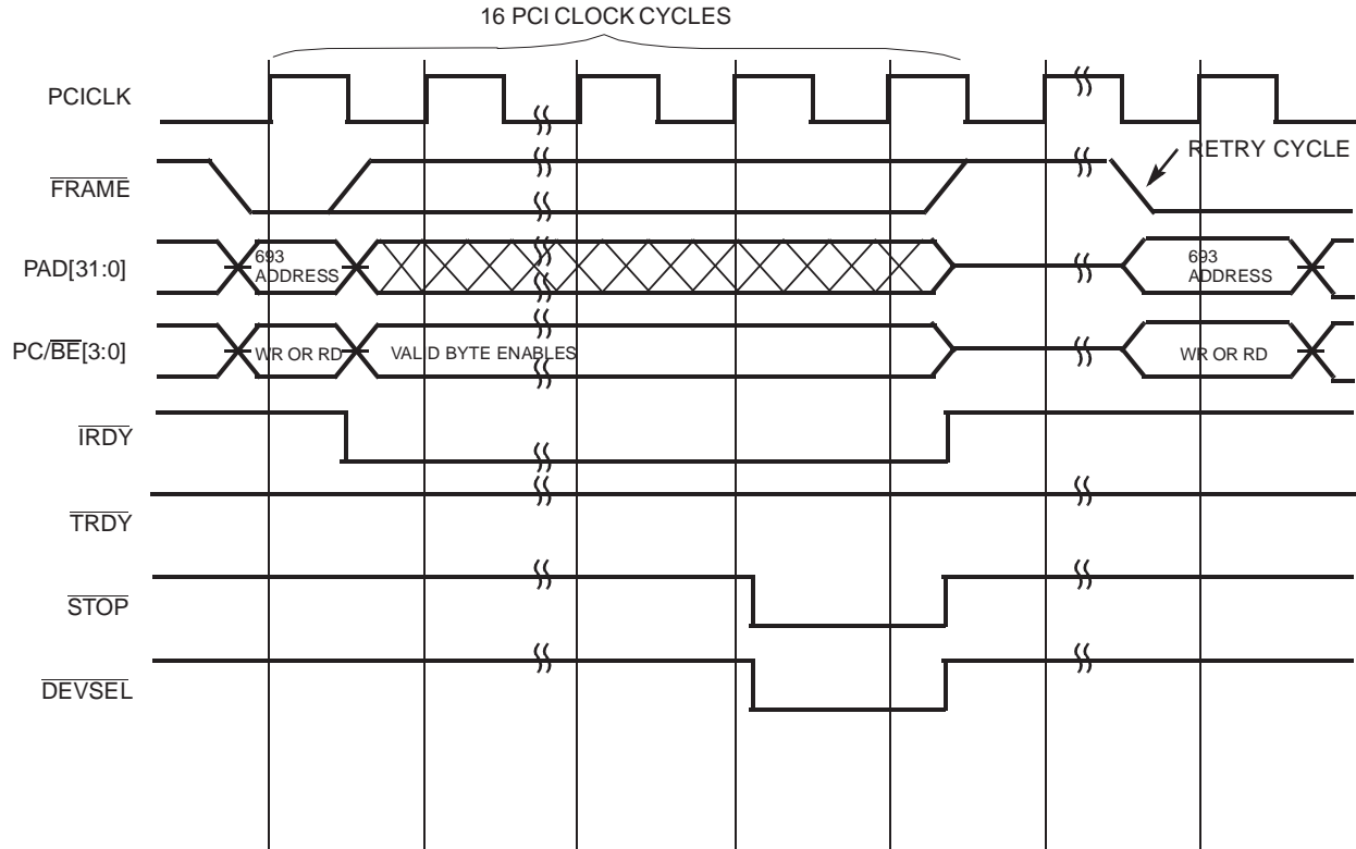
693 Generated Retry (For Accesses Requiring More Than 16 PCI Clock Cycles to Complete)
