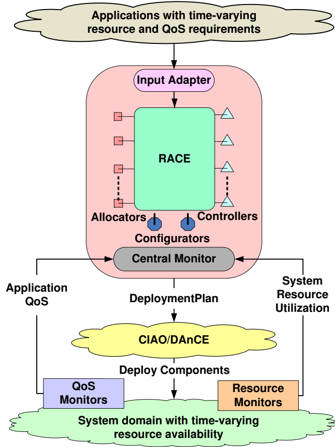
Figure 4: Detailed Design of RACE
