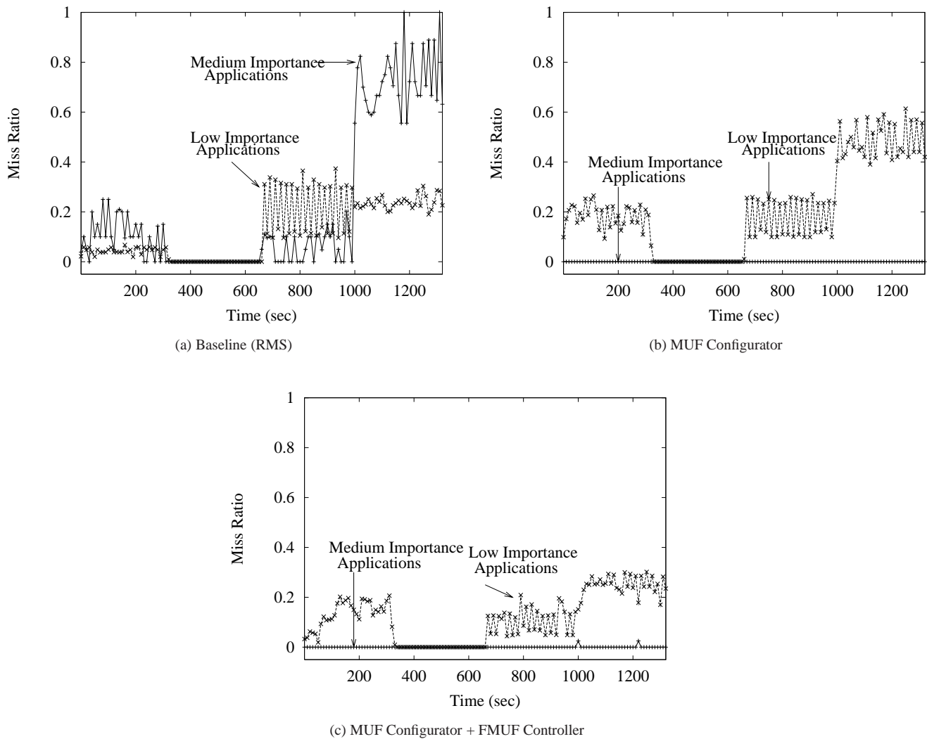
Figure 12: Deadline Miss Ratio Under Moderate Workload
