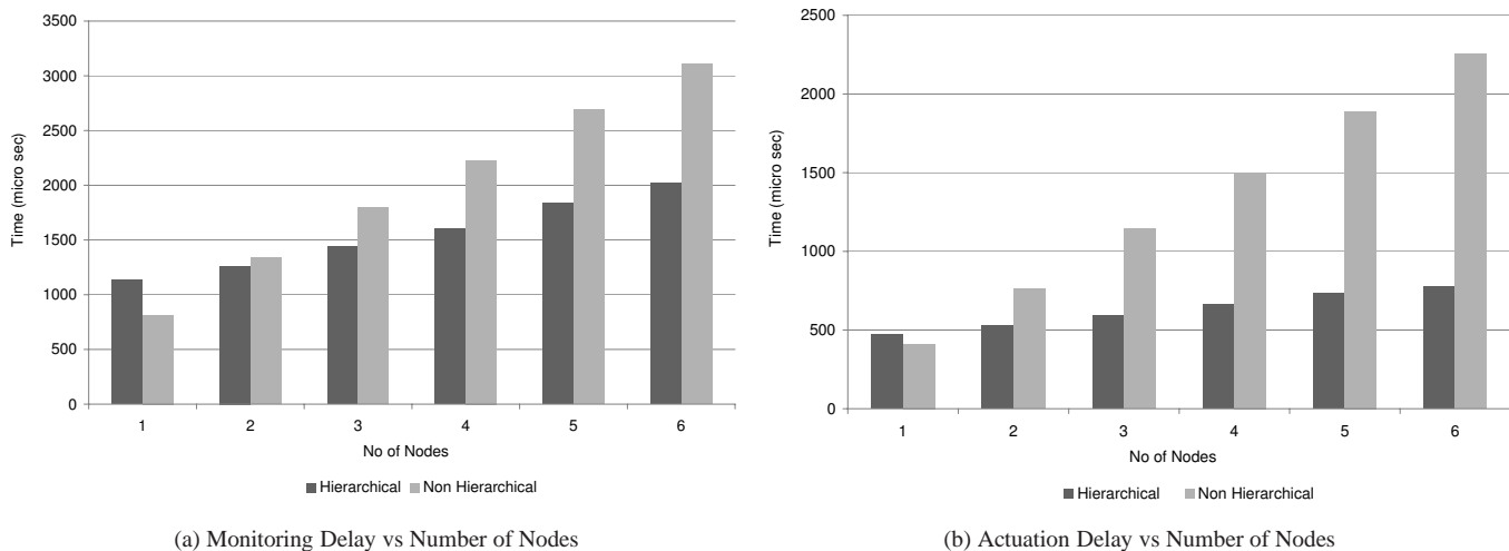
Figure 10: Impact of Increase in Number of Nodes on Monitoring and Actuation Delay
