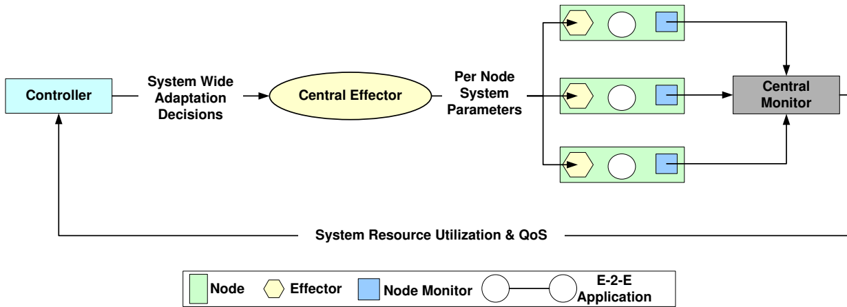
Figure 9: RACE's Feedback Control Loop
