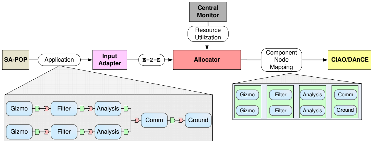
Figure 5: Resource Allocation to Application Components Using RACE
