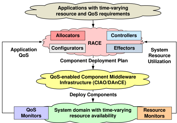
Figure 1: A Resource Allocation and Control Engine (RACE) for Open DRE Systems
